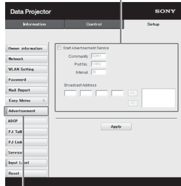
Кнопка Advertisement
