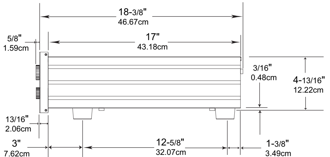
Side View of the C500C
