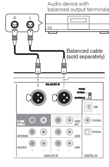
A-70DA's rear panel
