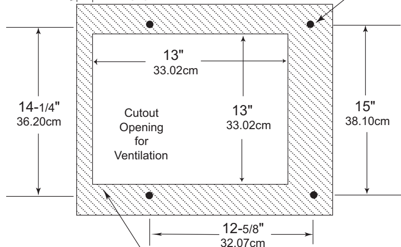
MX120 Bottom View in Custom Cabinet
