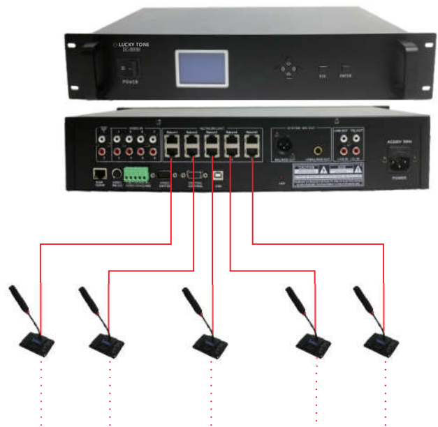
DC-800M Main Control Unit
