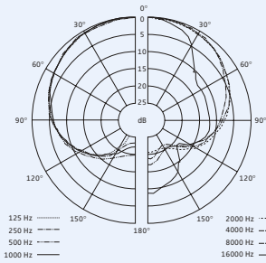
Polar diagram MME 865-1
