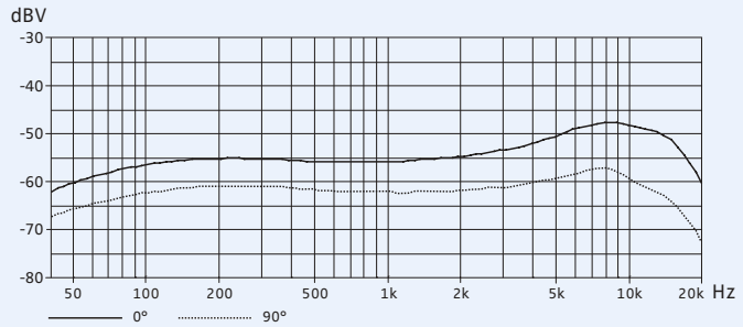
Frequency response curve MME 865-1
