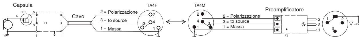
Schema circuitale
