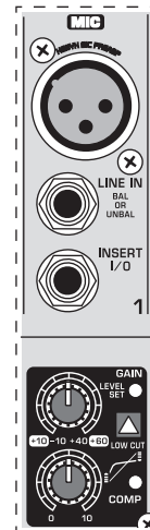
Fig. 2.1: Connectors and controls of mic/line inputs
