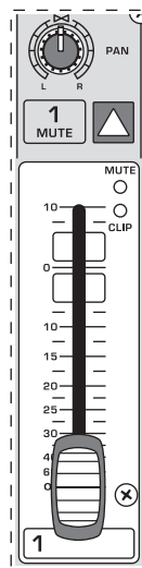
Fig. 2.4: Channel fader and additional control elements
