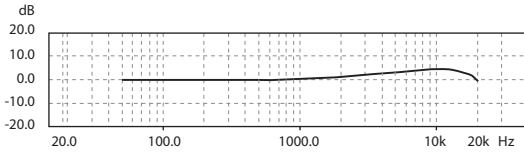
Frequency response
