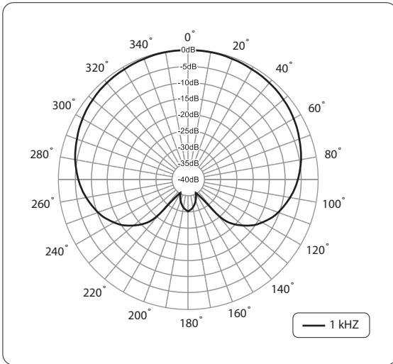
Polar pattern
