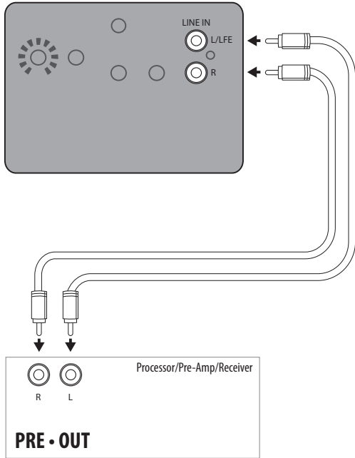
Left and Right pre-outs on Processor/Pre-Amp/Receiver connected to Left and Right line inputs on subwoofer amplifier
