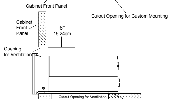
MVP901 Side View in Custom Cabinet
