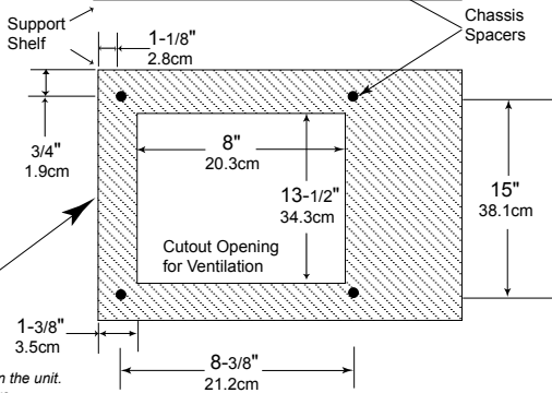
MVP901 Bottom View in Custom Cabinet
