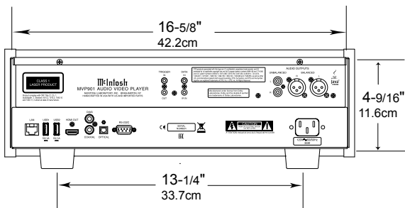
Rear View of the MVP901
