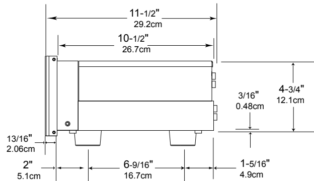
Side View of the MVP901
