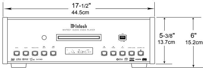
Front View of the MVP901
