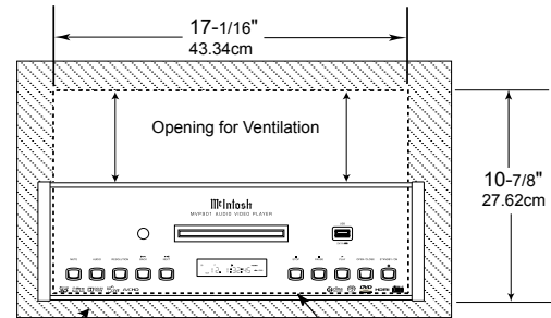
MVP901 Front Panel Custom Cabinet Cutout
