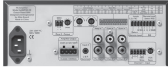
AA50PHD-CE - REAR
