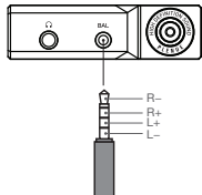
Pin Arrangement of Balanced Audio Port (2.5mm 4-pole)
