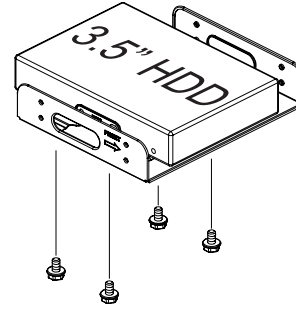
Bolt A
