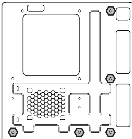
ATX Board
