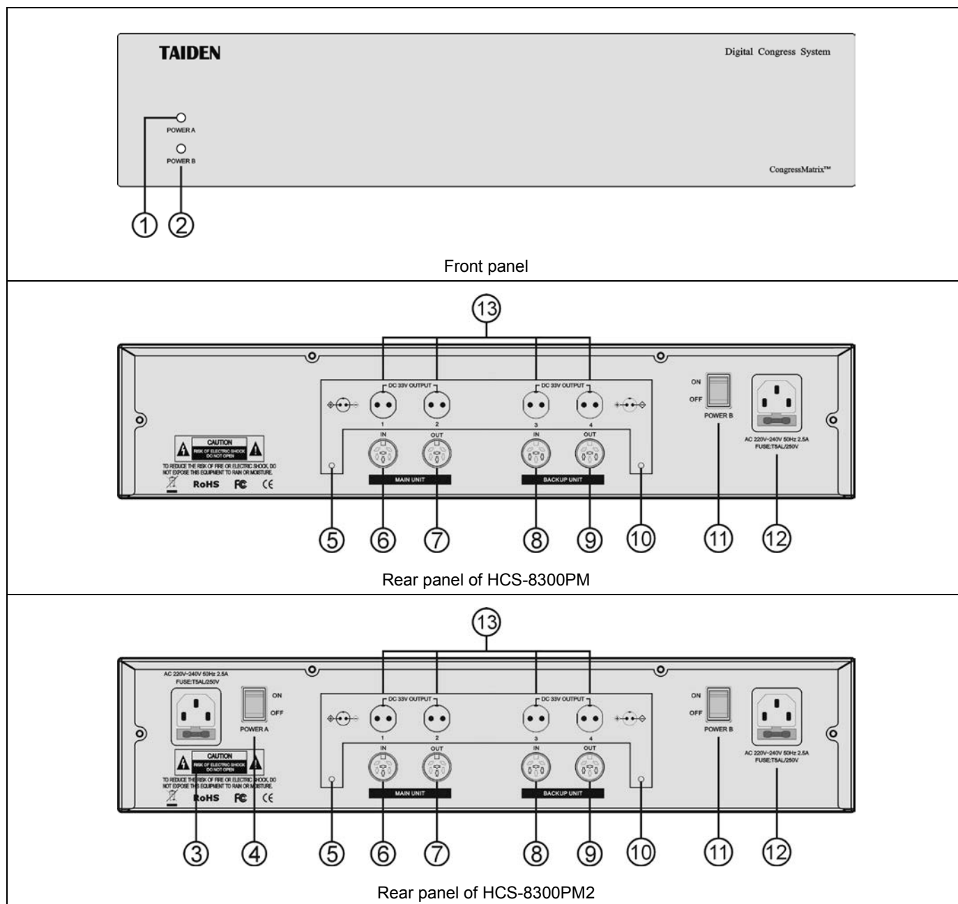
Figure 6.9.1 Power Supply Unit
