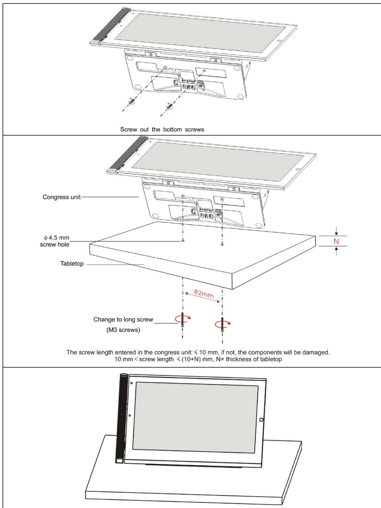
Figure 3.2.2 Fixed installation of HCS-8368/50 series congress unit
