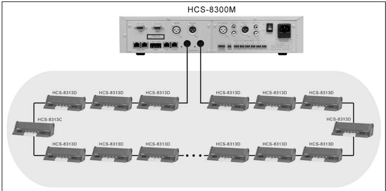
Figure 1.1.11 “Closed Loop - Daisy Chain” connection topology
