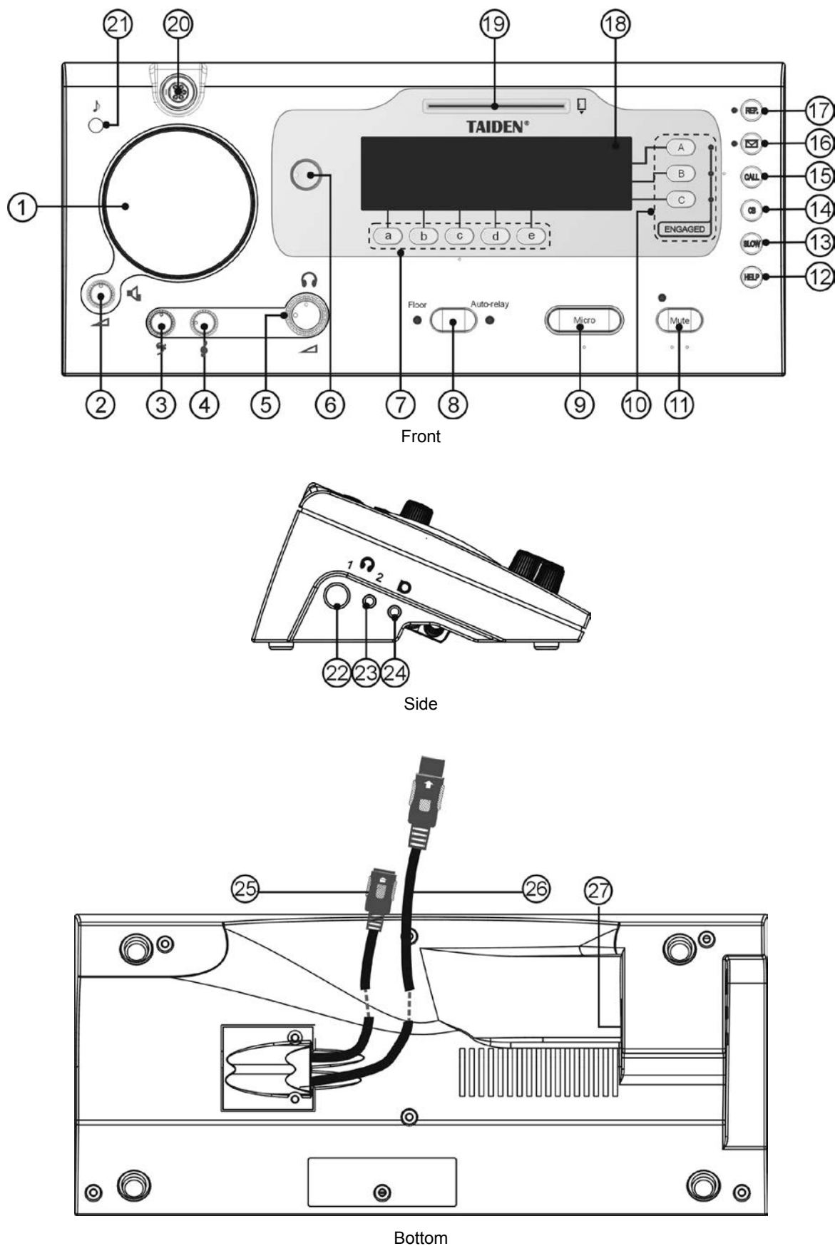
Figure 4.1.1 HCS-4385U/50 Interpreter unit
