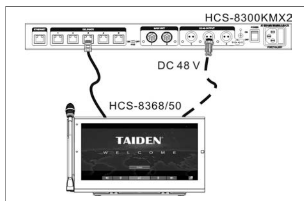
Figure 3.2.6 HCS-8368/50 series paperless multimedia congress terminal connecting to HCS-8300KMX2 Ethernet switcher (not PoE)
