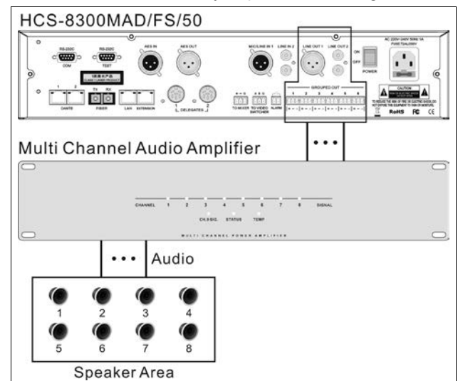
Figure 2.1.7 CMU connecting to PA
