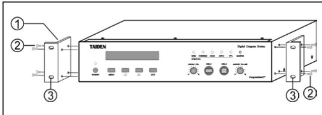
Figure 2.1.3 Installation of the CMU
