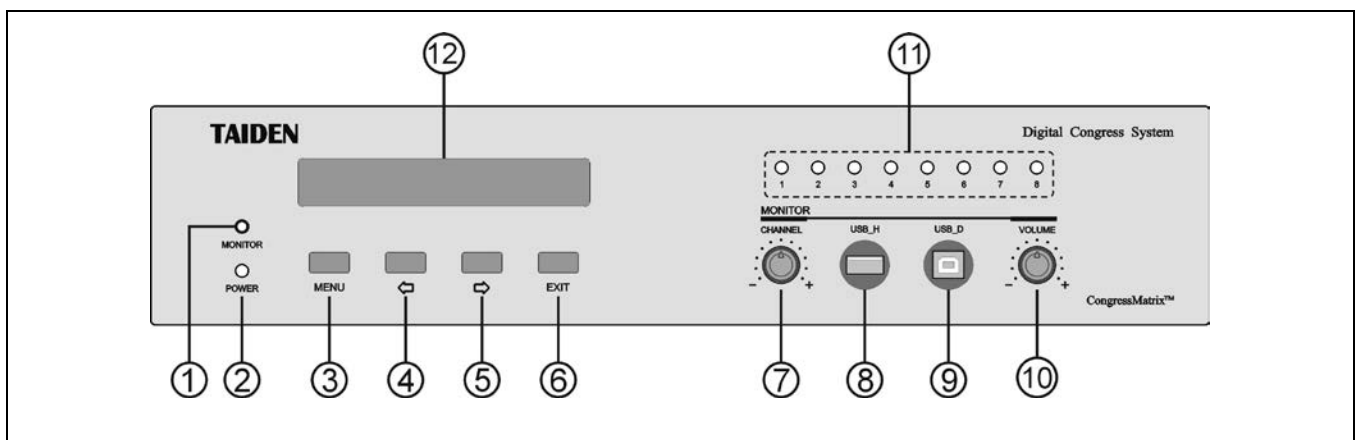
Figure 6.1.1 Front panel of HCS-8300MO Series 8 Channels Audio Output Device
