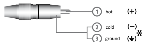
RCA IN Jack (unbalanced)
