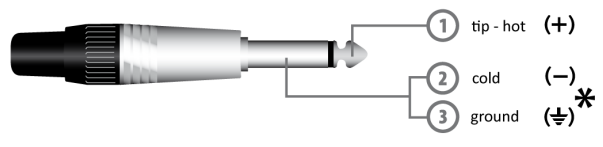
LINE IN, various OUT Jack (unbalanced)
