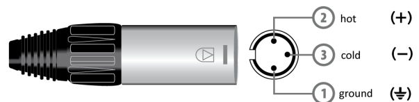
MIC INPUT Balanced male XLR
