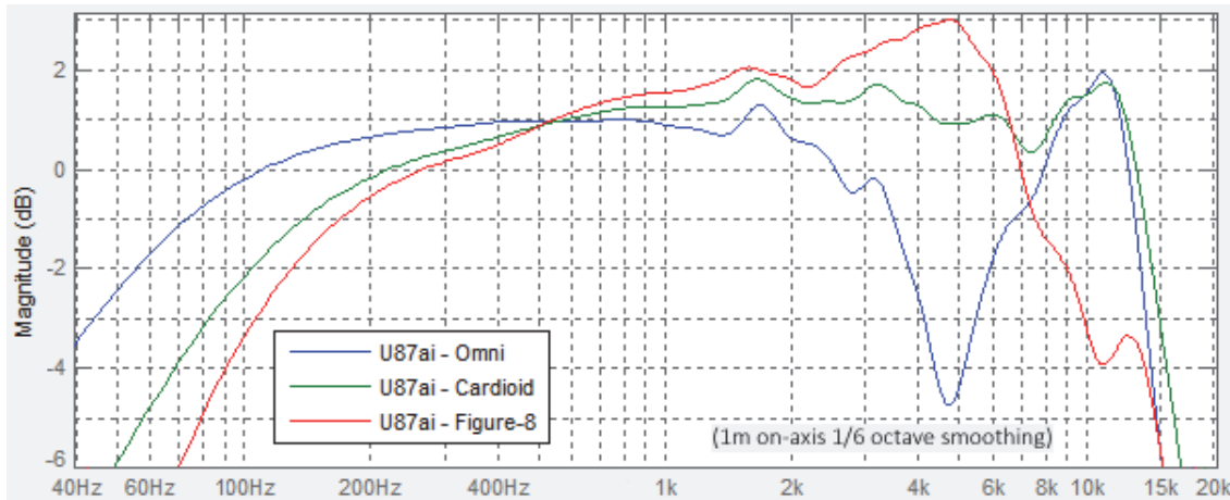
Figure 5-3 U87ai measured on-axis frequency response
