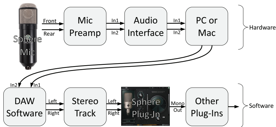
Figure 4-1 Sphere signal chain with mono output plug-in
