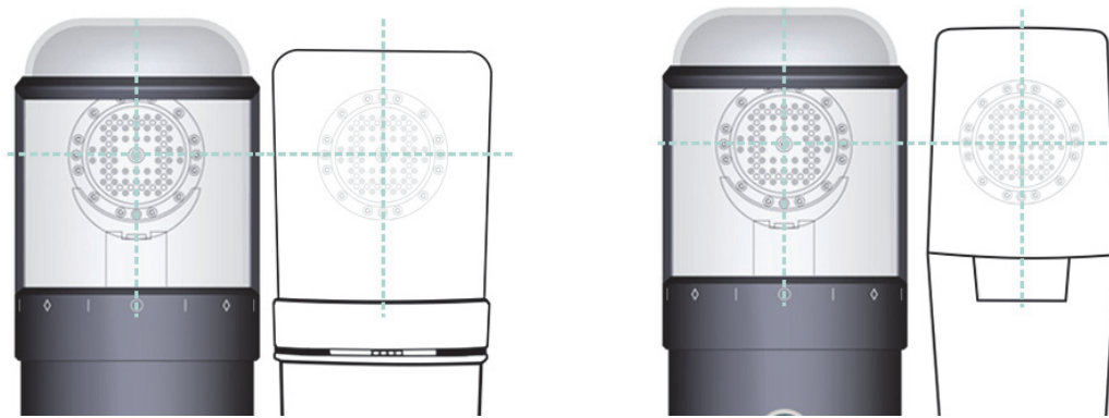
Figure 4-3 Lining up capsule centers for Sphere and Neumann U67/U87 (left) and AKG C414 (right)
