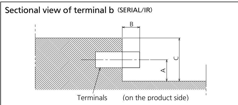
Terminal b 49SF1HW Terminal (Side)
