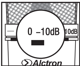
The pad switch helps prevent distortion from extremely loud sources, such as when close-miking horns or drums.
