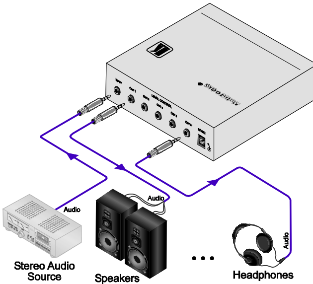
Figure 8: Connecting the VM-50HN Headphone Distributor
