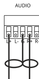
Figure 5: Connecting to an Unbalanced Stereo Audio Acceptor
