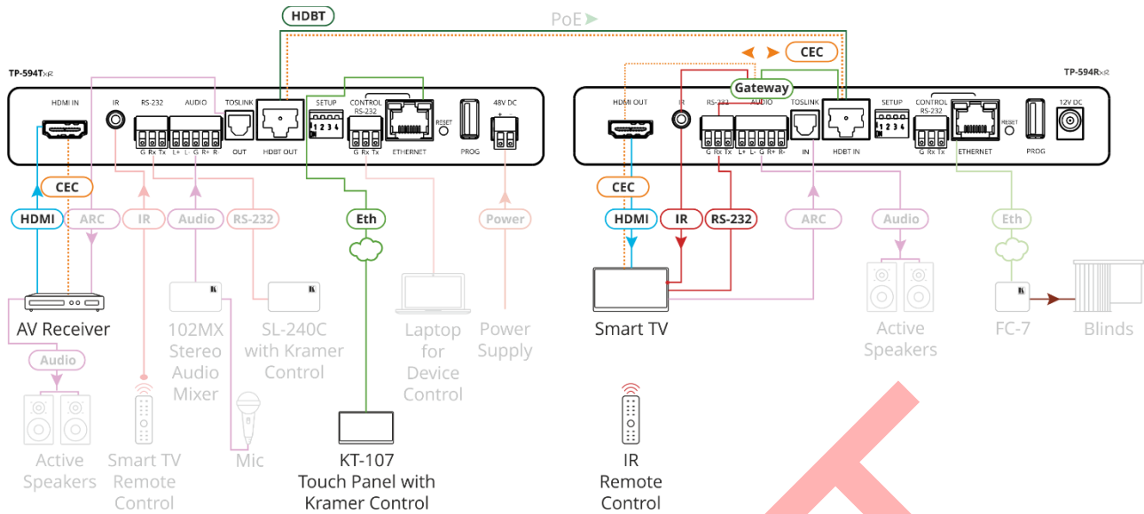
Figure 22: Extending Signals via Control Gateway
