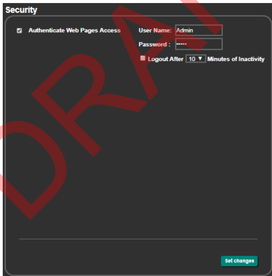
Figure 47: Security Page
