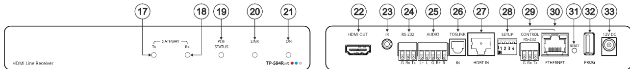
Figure 2: TP-594Rxr HDMI Line Receiver
