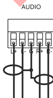
Figure 4: Connecting to a Balanced Stereo Audio Acceptor
