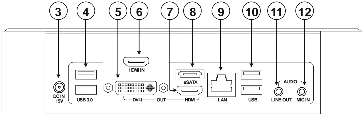
Figure 3: VIA Campus PLUS Rear Panel
