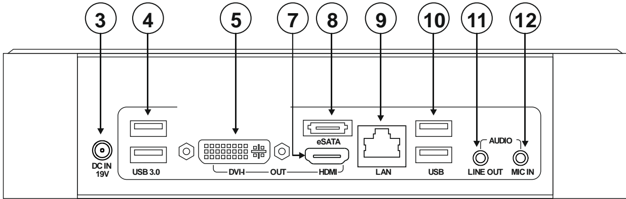
Figure 2: VIA Campus Rear Panel
