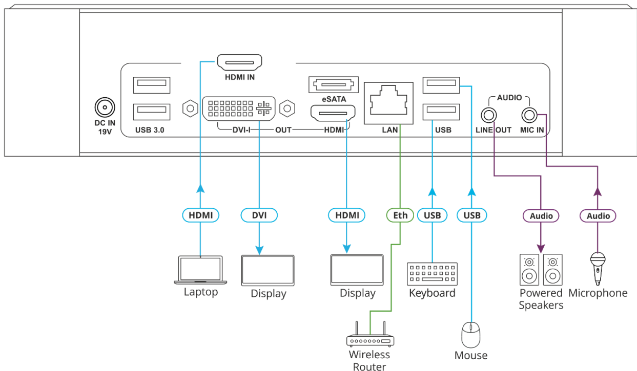
Figure 4: Connecting to the VIA Campus PLUS Rear Panel
